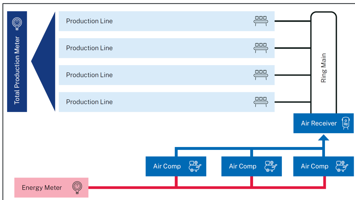
Figure 8: An illustration of the Compressed Air System (CAS) before the NRE.
