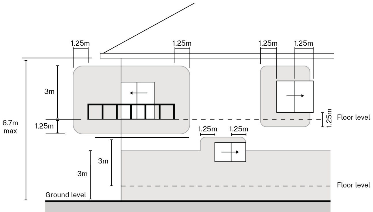
Figure 3-6 Unsuitable points of attachment shown shaded
