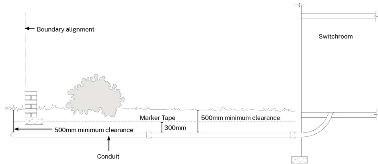
Figure 2-4 Typical service conduit – non-domestic
