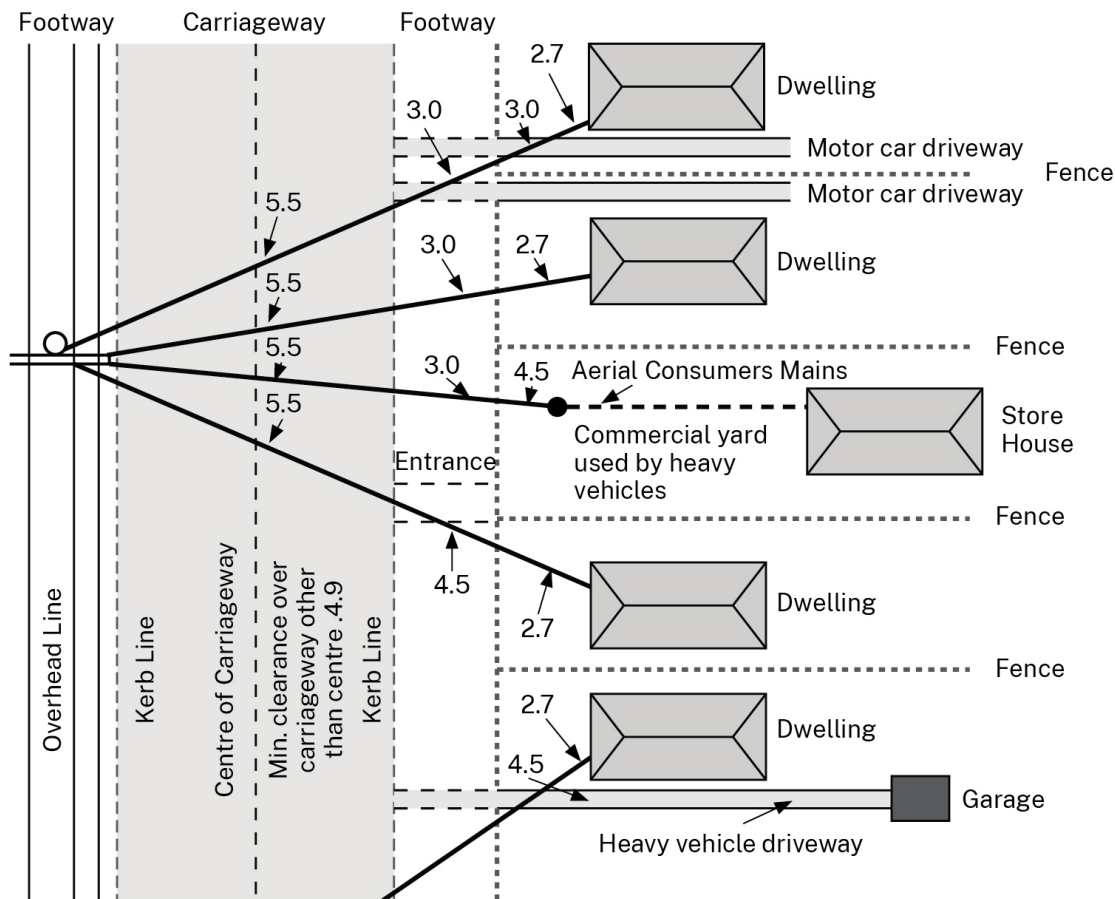
Figure 3-3 Typical clearance situations – plan
