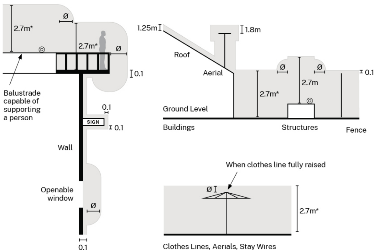
Figure 3-2 Typical clearance situations – elevation
