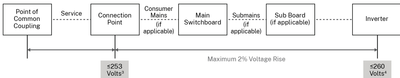
Figure 8-3 Voltage rise limits for installations with embedded generation
