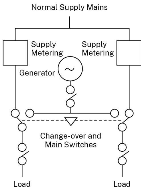
Figure 8-2 Changeover switches
