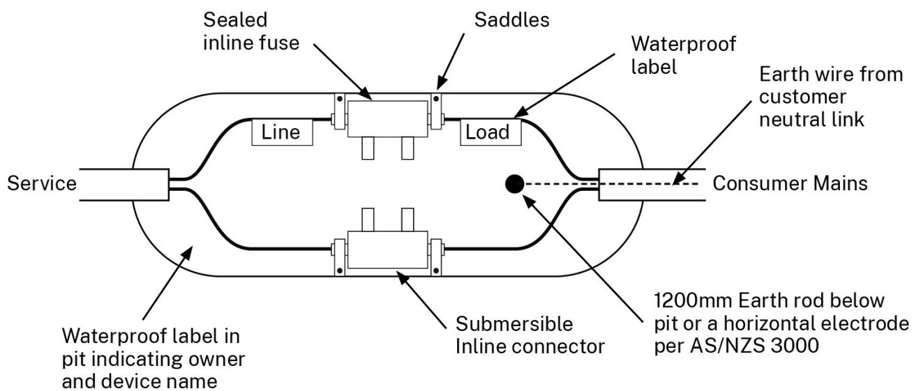
Figure 5-6 Example of pit using sealed inline fuse and insulation piercing connectors
