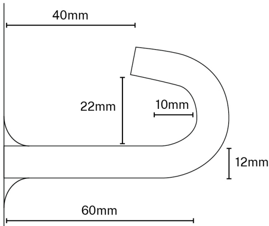
Figure 3-9100-A service hook
