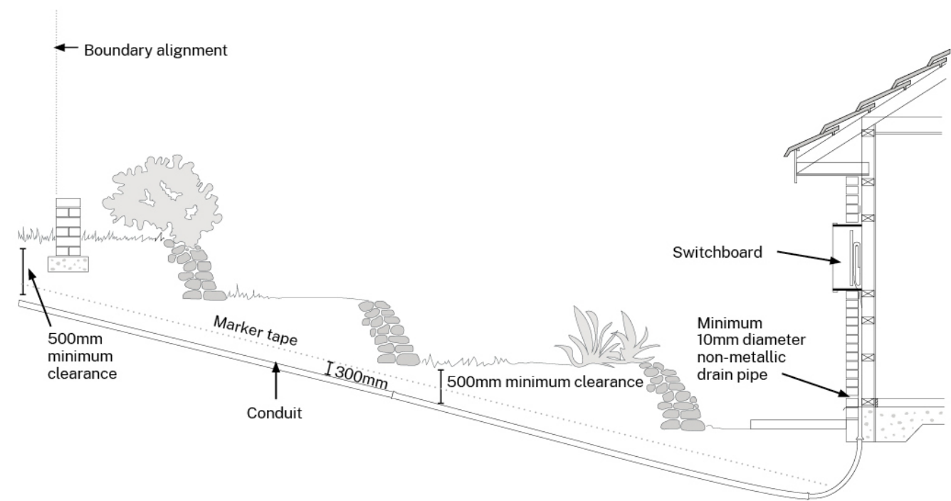
Figure 2-3 Typical service conduit in domestic premises
