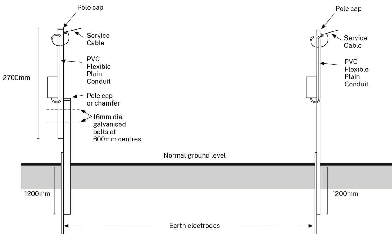
Figure 3-10 Typical builder's service
