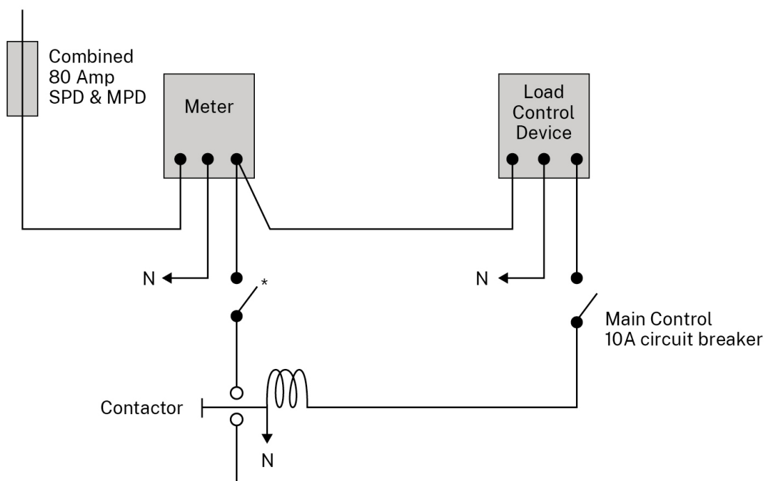
Figure 4-3 Controlled load – contactor wiring
