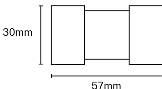
Figure 4-2 100A fuse link dimensions
